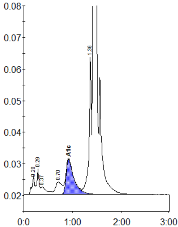
Peak table - ID: 10508798
